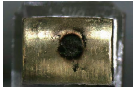
Fixed contact
