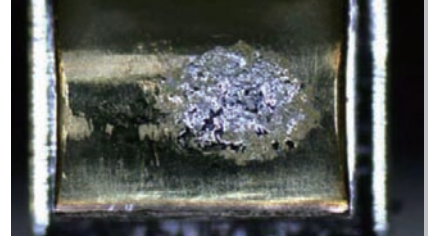
Fixed contact
