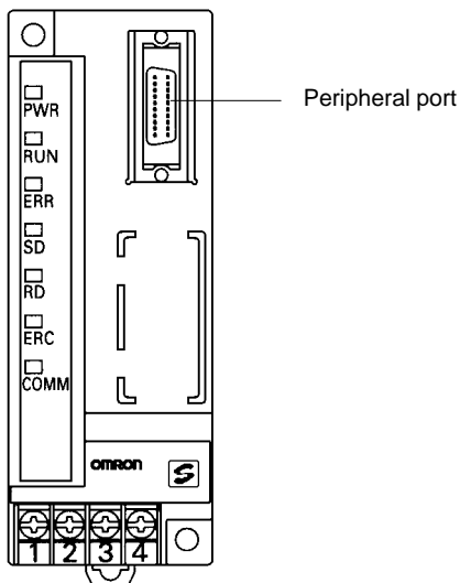
SRM1-C01-V2 (No RS-232C port)
