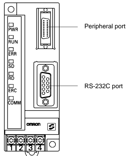
SRM1-C02-V2 (With RS-232C port)
