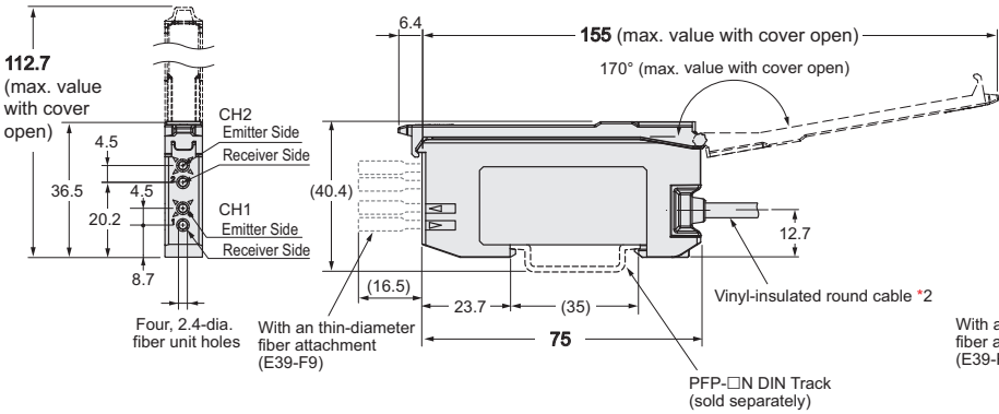
Mounted to DIN Track
