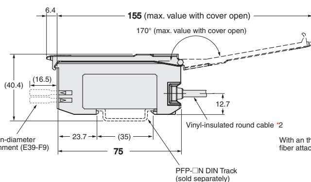
Mounted to DIN Track
