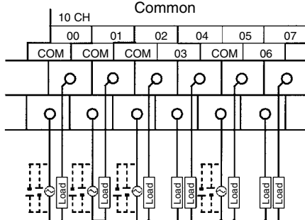
CPM1A-20CDR-□(-V1)/CPM1A-20EDR/20EDR1
